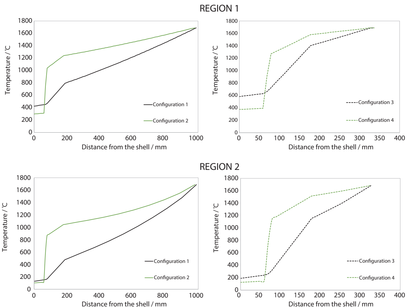
Fig. 3 Thermal profile along the material.
