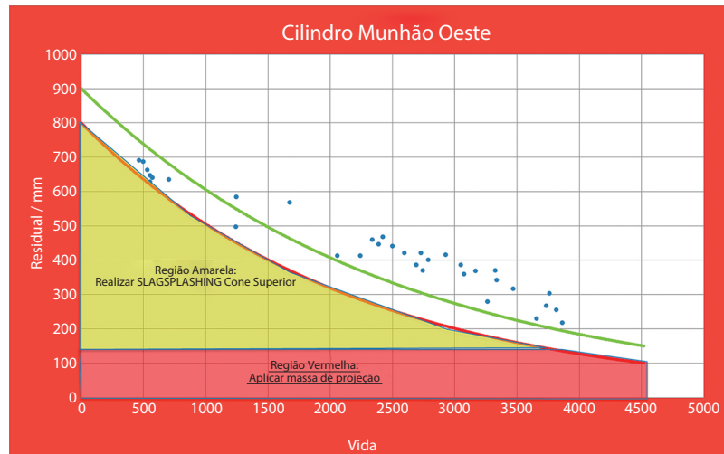
Fig. 7 Trunnion wear curve.
