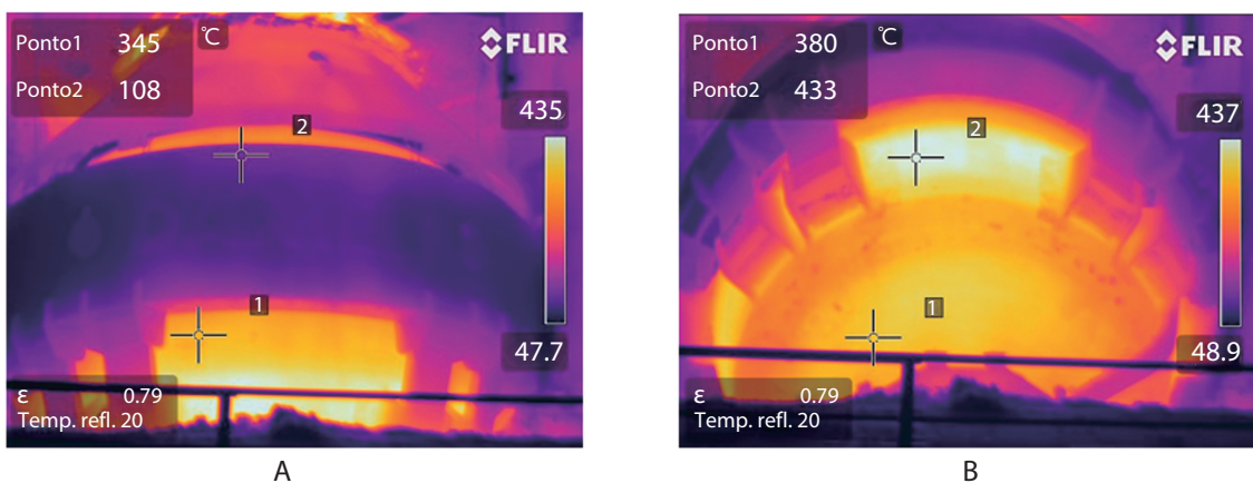
Fig. 5 Thermography performed on BOF with 400 heats.
