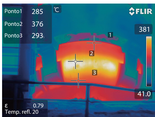
Fig. 6 Thermography of BOF#4 with 4000 heats.
