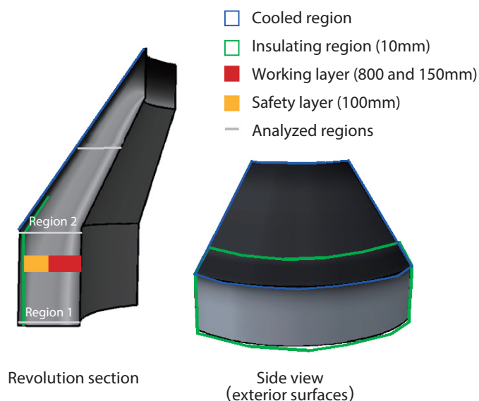
Fig. 1 Cross-section and lateral view of the studied problem 1) .
