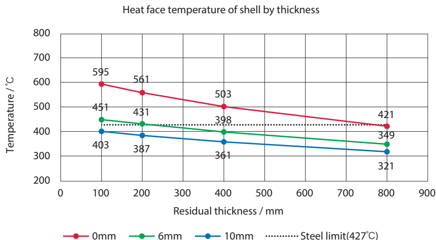
Fig. 4 Evaluation of final shell temperature as a function of residual thickness.
