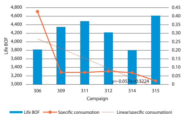
Fig. 9 Evolution campaigns.
